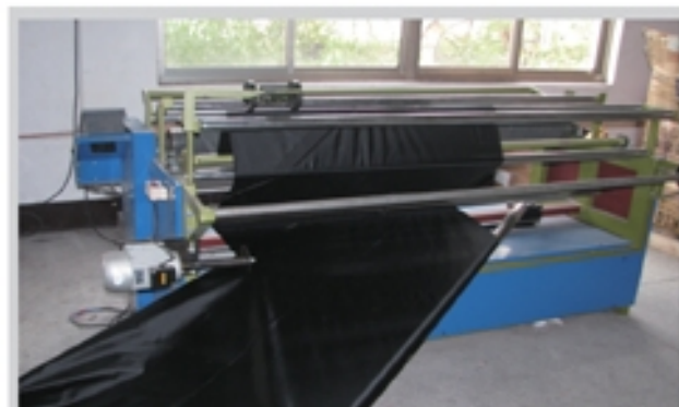
Fabric Bias Cutting Machine 面料热斜裁机
